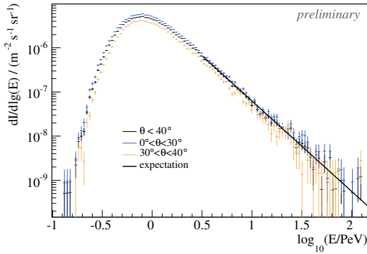
Figure 4: Preliminary, raw energy spectrum without acceptance correction. The difference between high and low zenith range indicates the systematic uncertainty. Though not deconvoluted yet, the slope of the high-energetic part already agrees well with the expected spectrum (solid line, [7]).
