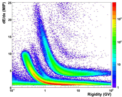
Figure 4: Distribution of the mean rate of energy loss in the silicon sensors of the tracking system, as a function of the particle rigidity, for a sample of positively charged cosmic rays. Moving from bottom-left to top-right, the following particle species can be recognized: e^+ , p and d, ^3\text{He} and ^4\text{He} , Li, Be, B and C
