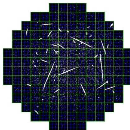
Fig. 3 Images of simulated air shower events on the focal surface with 10^{20} eV and various incident angles. Fifty events are super imposed. (EC : blue line, PDM : green line)
