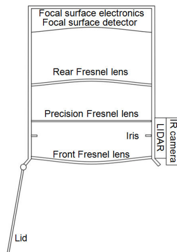
Fig. 1 Configuration of the JEM-EUSO telescope
