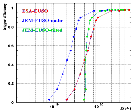
Fig. 5 Trigger efficiencies vs. energy for ESA-EUSO(min) (red line) and JEM-EUSO (vertical mode: blue line and tilt mode: green line)
