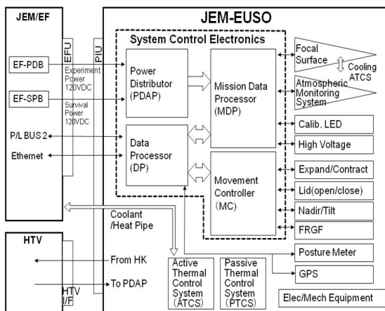
Fig. 4 Block diagram of the JEM-EUSO system functions
