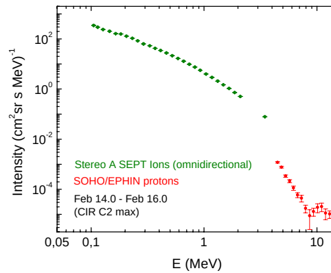
Fig. 5. CIR energy spectrum (mostly protons)
