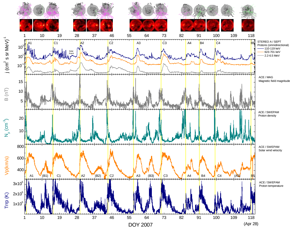
Fig. 4. CIR accelerated proton events during 2007
