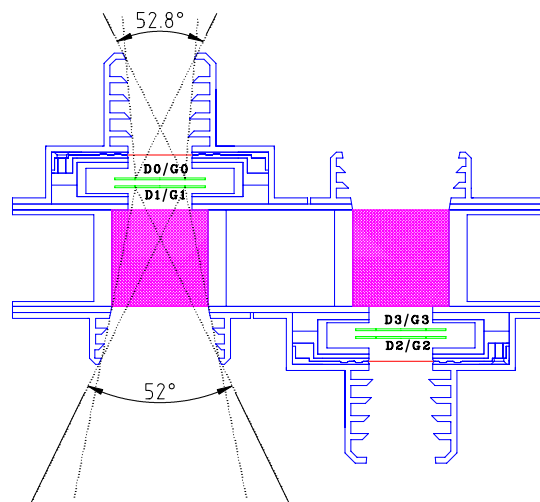
Fig. 1. SEPT sensor schematics. Detection elements are silicon detectors (D0...D3, green) with guard rings (G0...G3), Parylene foils (red), and magnetic fields perpendicular to the drawing plane (magenta).
