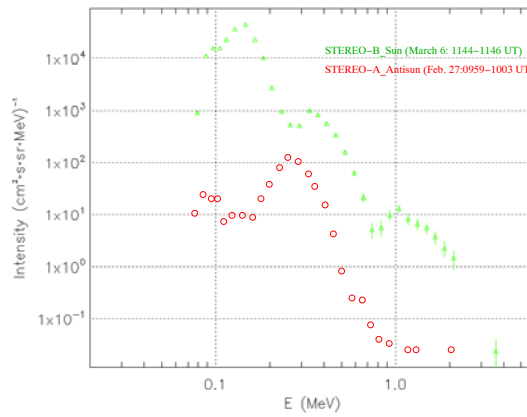
Fig. 3. Peculiar energy spectra of upstream events. STEREO-A looking towards Earth/anti-sun and STEREO-B looking towards Earth/sun.
