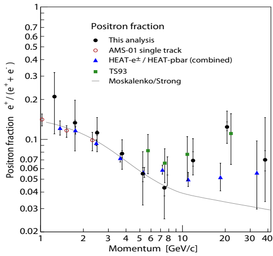
Figure 4: The positron fraction e^+/(e^+ + e^-) measured in this analysis (filled circles), compared with earlier results from AMS-01 (open circles) [10], TS93 (squares) [2], the combined results from HEAT- e^\pm and HEAT-pbar (triangles) [1], together with a model calculation for purely secondary positron production from [12] (solid line). The total error is given by the outer error bars, while the inner bars represent the systematic contribution to the total error.
