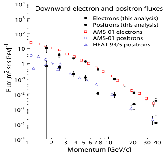
Figure 5: The fluxes of downward going positrons (filled circles) and electrons (filled squares) measured in this analysis, compared with earlier results from AMS-01 (open circles and squares) [10] and HEAT- e^\pm (triangles) [5]. Error bars denote statistical errors only.
