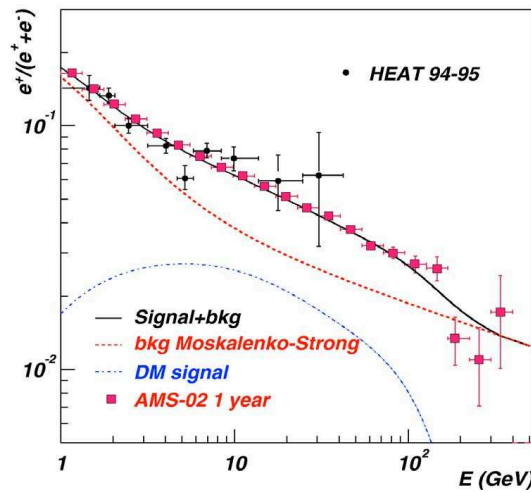
Figure 6: Expected positron fraction measurement with one year of AMS-02 data [14].
