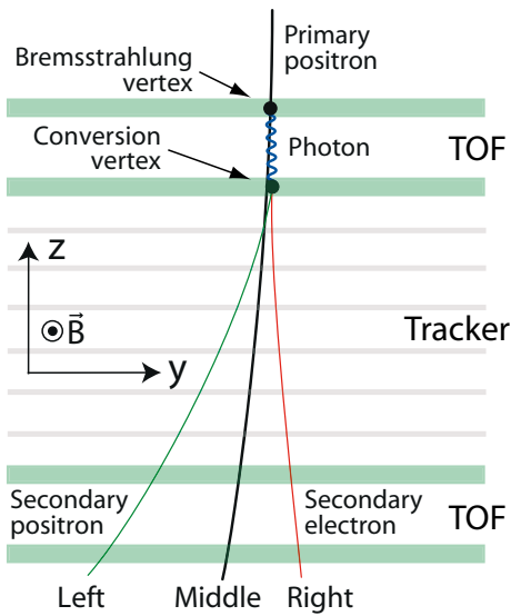
Figure 1: Schematic view of a converted bremsstrahlung event caused by a positron going top-down.
