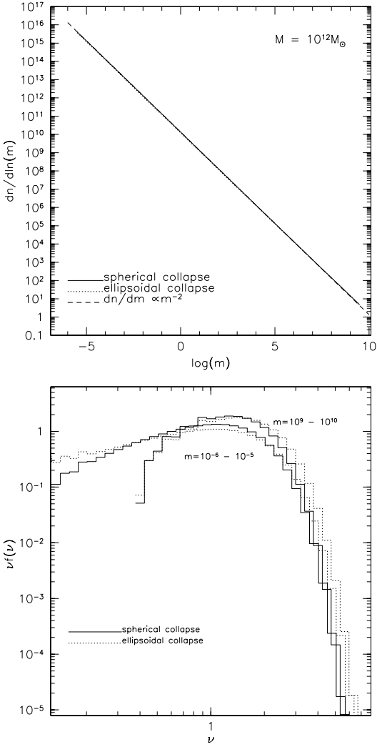
Figure 1: Upper panel: differential distribution of subhalos in a 10^{12} M_\odot/h DM halo. A least-squares fit on the points gives \alpha_{sc} = -0.9972 \pm 0.0001 and \alpha_{ec} = -0.9937 \pm 0.0003 for the spherical and ellipsoidal collapse model, respectively. Lower panel: subhalo distribution in term of \nu = \delta_{sc}/\sigma(m) for the smallest and biggest decades of mass considered in the analysis.
