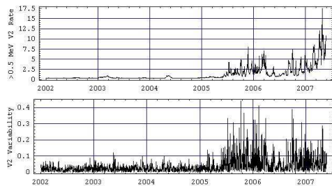
Figure 2. Low-energy count rates and their day-to-day variability for Voyager-2.
