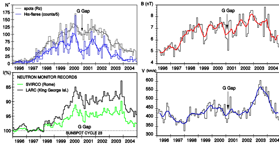
Figure 1: Monthly time history of sunspot and flare numbers (upper left panel), neutron monitor records (lower left panel), solar wind speed (lower right panel) and interplanetary magnetic field intensity (upper right panel) during the current solar activity cycle. Thick trends show the 5-month running averages (note the wave trends). Arrows refer to the Gnevyshev Gap identification.
