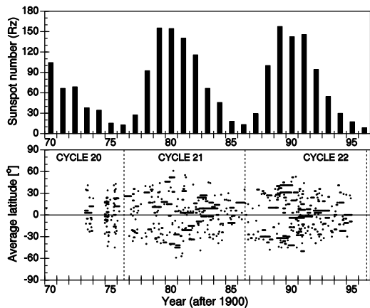
Figure 3: Isolated CH distribution in latitude, derived from data reported by NOAA (bottom) and yearly sunspot number (upper panel).
