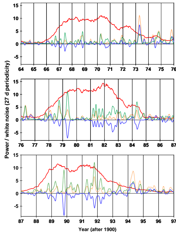
Figure 2: Daily power to noise ratio of the 27-d periodicity for Kp (orange) and Dst (green) indices (blue trends give Kp-Dst power differences), together with the 27-d running averages of the sunspot areas (red; right scale in 10^{-6} Hemisphere).
