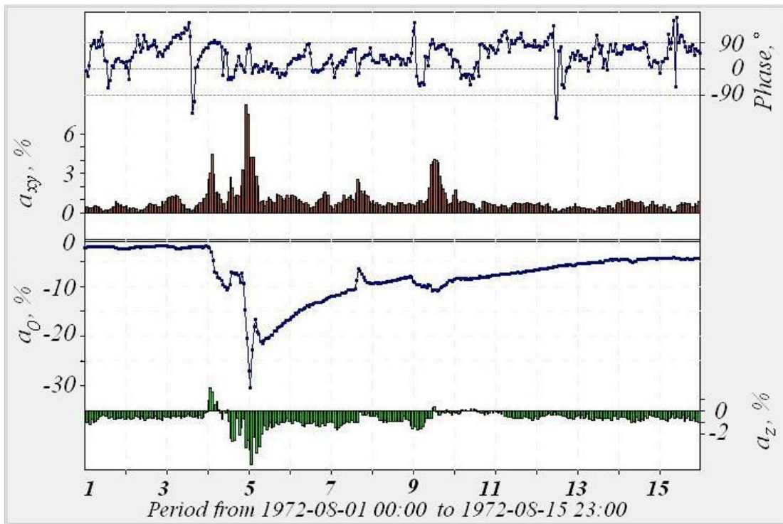
Figure 2. Behavior of all characteristics of CR Anisotropy in a graphical form.
