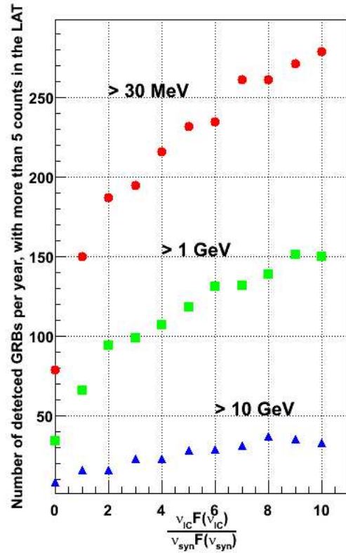
Figure 4: LAT sensitivity to GRBs for a self synchrotron Compton model as a function of the ratio of inverse Compton to synchrotron power outputs. Different curves refer to different energy thresholds.
