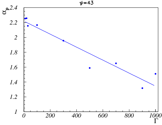
Figure 1: Correlation between \Gamma and the spectral index for \psi = 43^\circ . The correlation appears to be linear.
