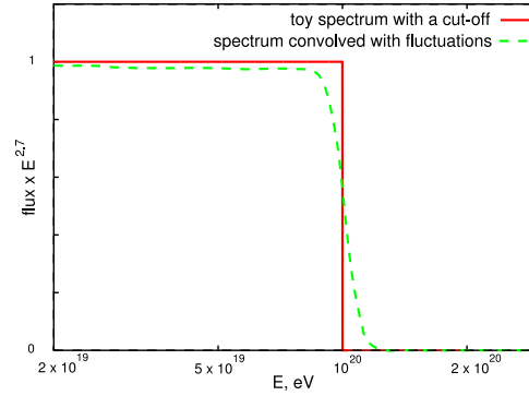
Figure 3: The impact of the small scale fluctuations on the toy primary spectrum with a cut-off. Dashed line shows the convolution of a toy spectrum and an energy estimation error presented in Fig. 2
