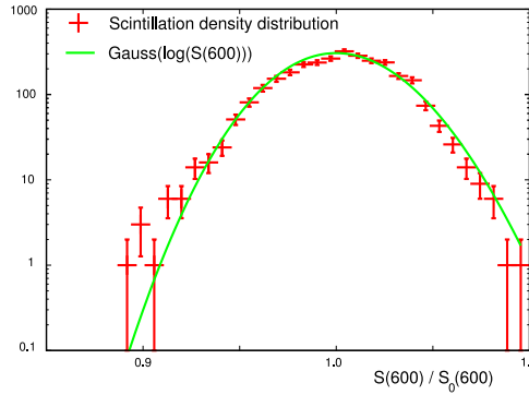
Figure 1: Scintillation density distribution over detectors (size of 14.8 \text{ m} \times 14.8 \text{ m} ) centered at [595 \text{ m}; 605 \text{ m}] core distance. Horizontal axis: scintillator density, normalized to average, vertical axis: number of detectors with a signal in a bin centered in S(600) (livni:18-3 shower).
