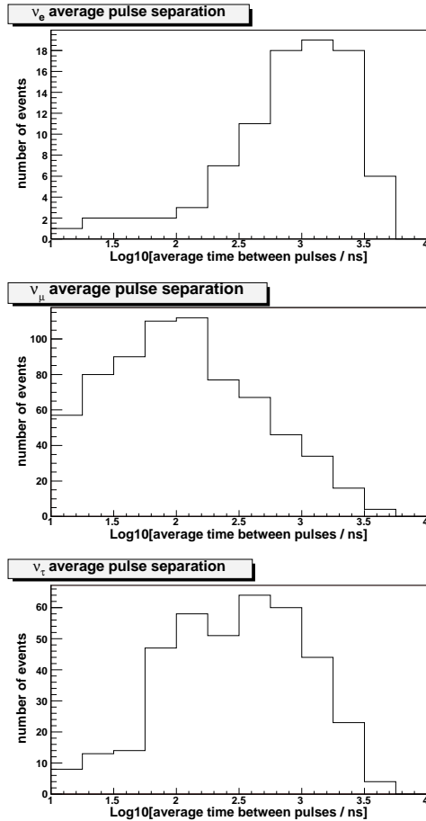
Figure 2: distribution of the average amount of time separating the pulses of a multiple bang event at 10^{20} eV. top: \nu_e , middle: \nu_\mu , bottom: \nu_\tau
