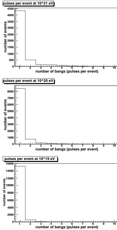
Figure 1: distribution of the number of pulses per event at 10^{21} (top), 10^{20} (middle), and 10^{19} eV (bottom)
