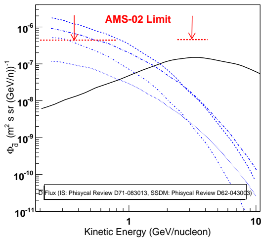
Figure 3: Estimated AMS-02 sensitivity limit for the antideuteron flux measurement compared to: the \bar{d} secondary IS flux [6]; the \bar{d} primary flux coming from the neutralino Dark Matter annihilation [3] for different points in the supersymmetric parameter space (labelled with a, b, c, d).
