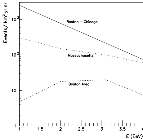
Figure 1: Expected rates versus energy for correlated events due to iron nuclei disintegrating on solar photons. This figure (with thanks to Alan Watson) is for events arriving from a direction close to the sun. The three lines show approximate rates characteristic of the separations attainable in different geographical areas (the Boston area, the entire state of Massachusetts, and a separation of roughly the distance from Boston to Chicago.)
