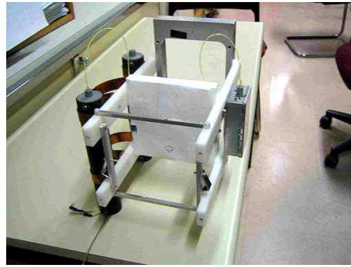
Figure 4: Scintillator ( 150\text{mm} \times 150\text{mm} \times 15\text{mm} from Kharkov, Ukraine with 1mm diameter Y11 wavelength shifter), exposed to 20 GeV muons at room temperature (22C) read out with a pixellated Geiger mode APD and PMT to produce the adjacent plots.
