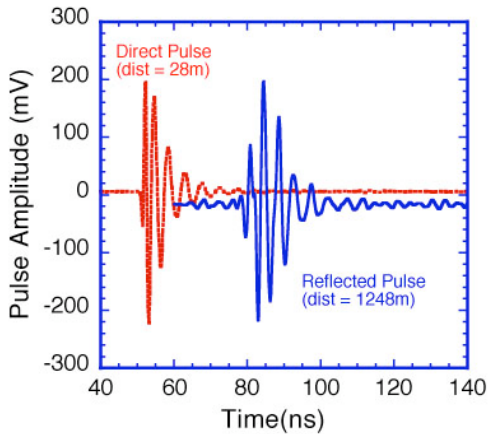
Figure 2: Comparison of radio pulses in the time domain. “Direct” pulse (left) propagated 28m through the air between transmitter and receiver. The right pulse was reflected from the bottom ice-water boundary. The time delay and amplitude is arbitrary.
