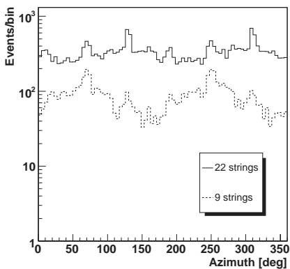
Figure 6: Azimuth distribution of atmospheric muons observed in the 9-string array in 2006 and the 22-string array in 2007.
