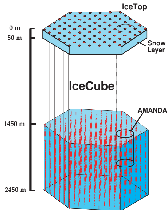
Figure 1: Schematic view of the IceCube array consisting of 80 strings with 60 sensors on each string. The surface array IceTop consists of 160 detectors, two of which are associated with each string.
