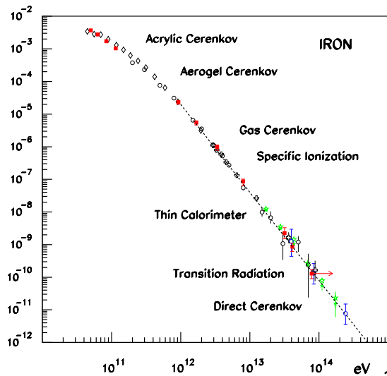
Figure 3: Iron energy spectrum above 10^{10} eV per particle in units of \text{m}^2 \text{ster}^{-1} \text{s}^{-1} , highlighting the complementarity between detection techniques. TRACER (red squares), HEAO-3 [2] (black diamonds), CRN [3] (black crosses), ATIC-2 [5] (black open circles), RUNJOB [6] (blue open circles) and HESS [8] (green stars).
