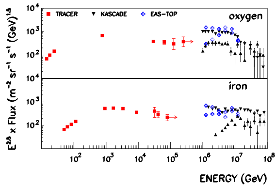
Figure 4: Energy Spectra from TRACER and from the interpretation of air shower data of KASCADE (for two different interaction models) and of EAS-TOPO (two data points for each energy are given, representing upper and lower limits). The spectra are for oxygen and for iron for TRACER, but for the “CNO-group” and the “Fe-group” for the other observations.
