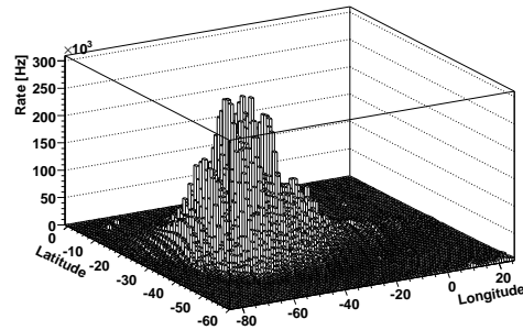
Figure 4: Singles rates (Hz) in the CAS1 detector as function of the orbital position averaged on several orbits traversing the SAA from South to North. The figure shows a detail of the rates in the vicinity of the SAA. Each bin in the histogram corresponds to the average rate in a 1 square degree.
