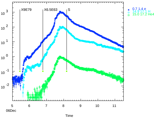
Figure 3. Shows electron, H, and He intensities observed by the Ahead HET for the first two events in December, 2006.
