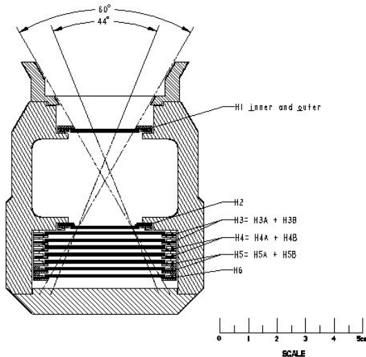
Figure 1: Cross-sectional view of the HET. For high rates the geometry factor for stopping particles is 0.61 \text{ cm}^2\text{-sr} .
