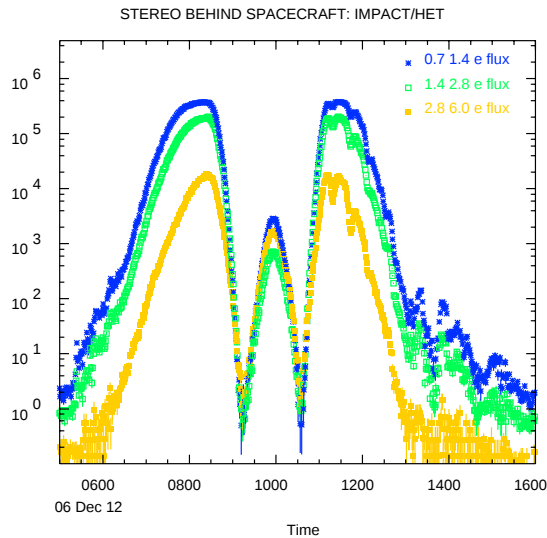
Figure 2. Electron intensities (electrons/cm 2 -sr-MeV) from the perigee passage of the Behind spacecraft of December 12, 2006.
