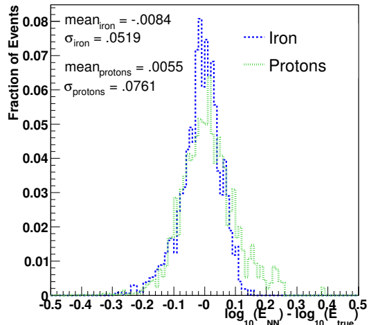
Figure 2: The energy resolution of the neural network for output energies between 1 and 10 PeV for proton and iron showers.
