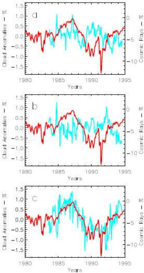
Figure 1: The graphs are from reference [5]. They show the global monthly cloud anomalies for a) high (< 440 hPa). b) middle (440 – 680 hPa) and c) (> 680 hPa) cloud cover (blue curve). To compute the monthly cloud anomalies the annual cycle is removed by subtracting the climatic monthly average (July 1983 - June 1994) from each month on an equal area grid before averaging over the globe. The global average of the annual cycle over this period for high, middle and low IR detected clouds is 13.5%, 19.9% and 28.7%, respectively. The cosmic rays (red curve) represent the neutron counts observed at Huancayo (cutoff rigidity 12.9 GV) and normalised to October 1965. The CR results extend over the whole period.
