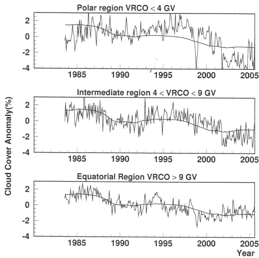
Figure 2: Cloud cover (spiky) compared with a best-fit sunspot number profile, including a slow droop in magnitude. VRCO is the vertical cut-off rigidity.
