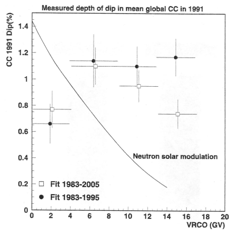
Figure 3: Comparison of the observed cloud cover modulation with that shown by the neutron count (normalised). The 'modulations' are expressed by the dip in the mean at the time of solar maximum (1991).
