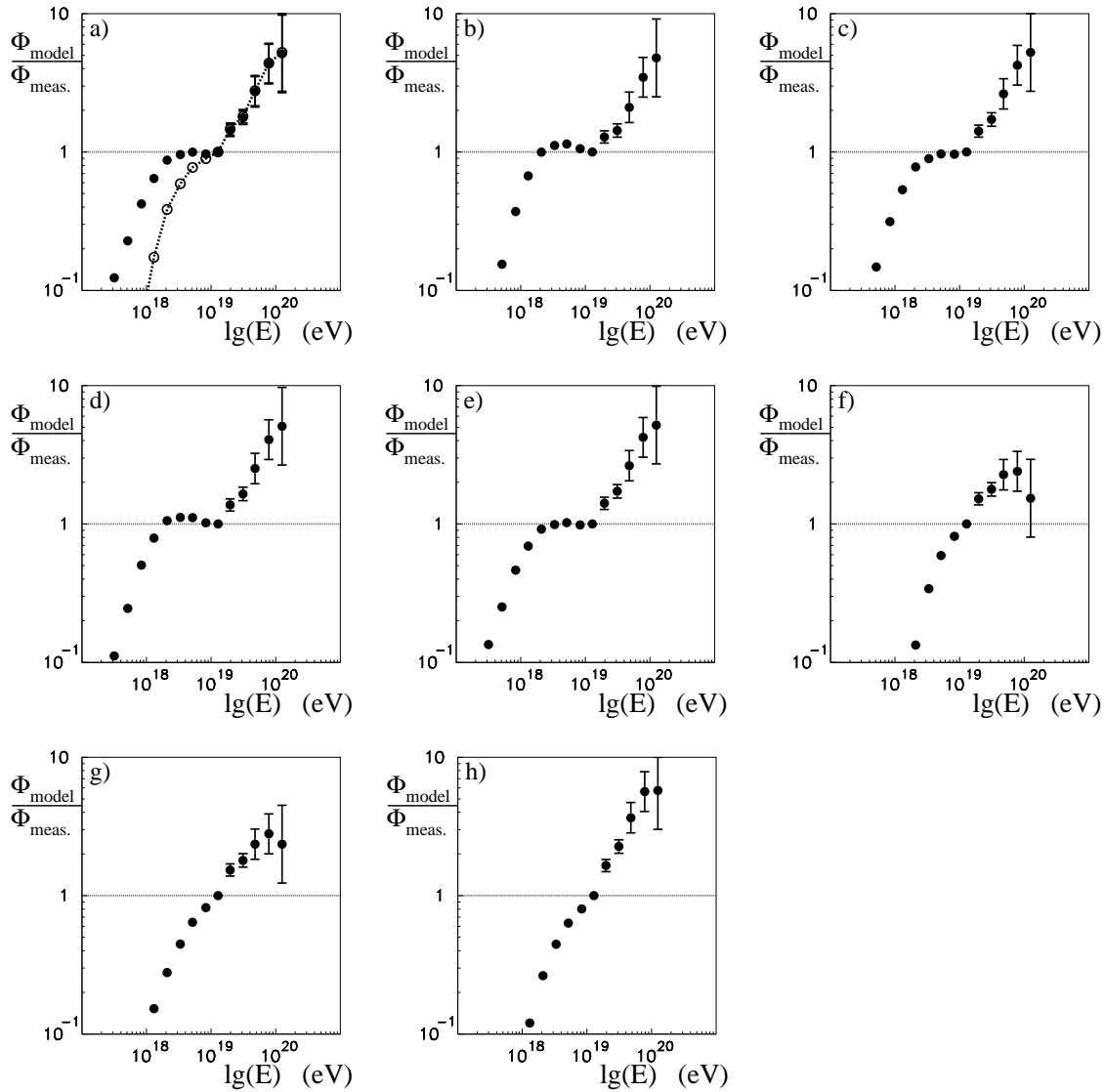
Figure 2: Ratios of predicted intensities to those measure from our previous summary, with the ‘low’ energy normalization for the models summarized in Table 1. In (a) the situation is also shown for there being no sources within 50 Mpc - dotted.
