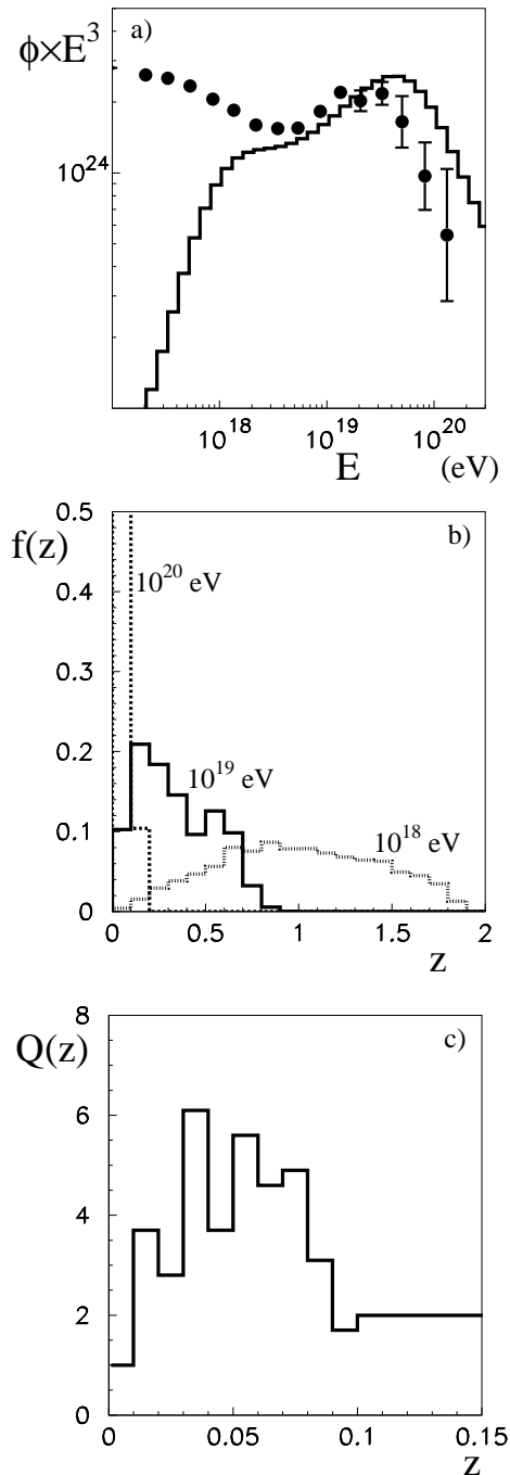
Figure 1: Results for the adopted galaxy cluster distribution (similar to that of AGN).
