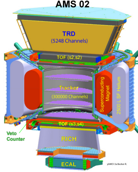
Figure 1. Full view of the AMS Spectrometer.
