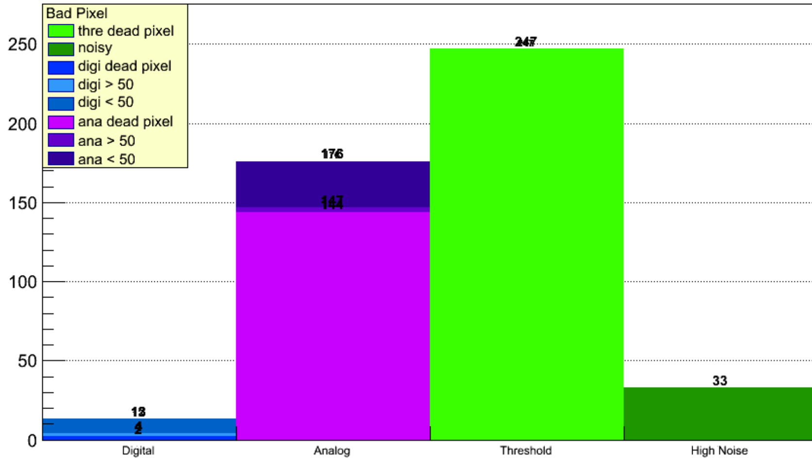
NumberBadPixelsOnStave
