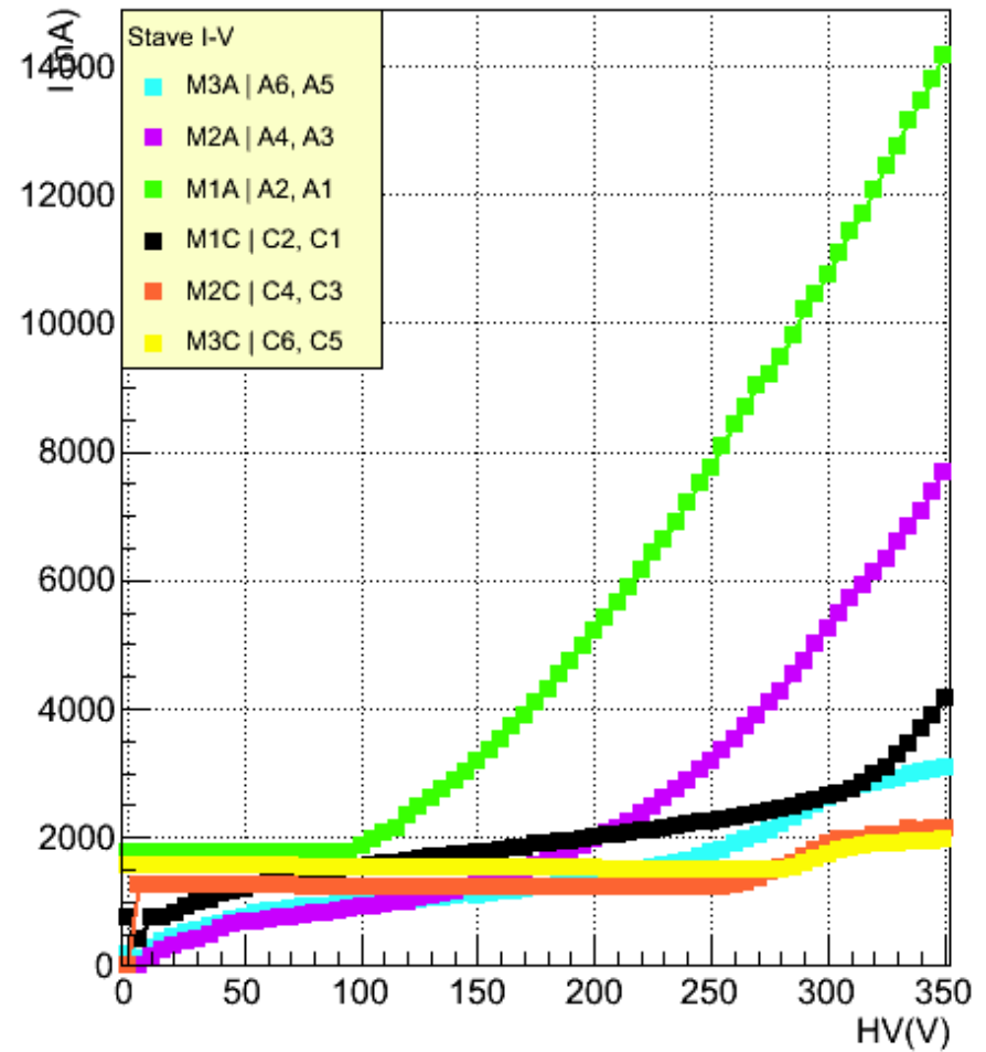
IV_planar
