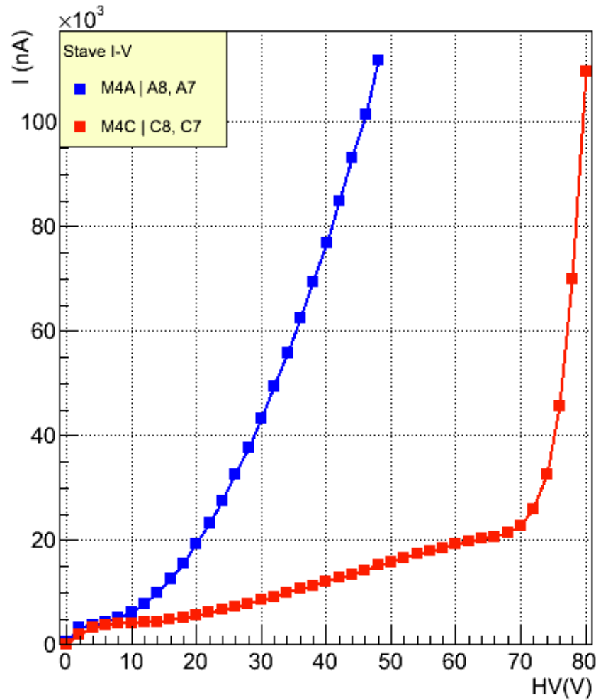
IV_3D
