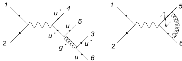
FIGURE 4.2: Working concept of MadLoop: generation of loop diagram (right) from L-cut diagram (left) obtained with MadGraph.
