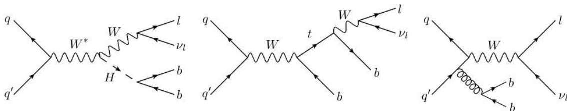
FIGURE 4.1: Example of processes containing a Wb\bar{b} final state: WH production (left), single top (middle), QCD Wb\bar{b} (right).
