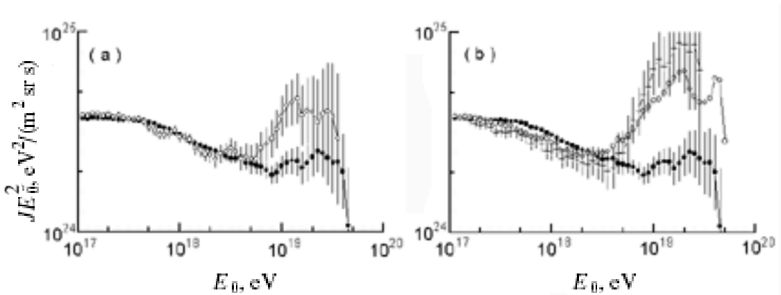
Figure 3. Integral energy spectra: \bullet for 22465 showers with the arrival directions outside of the equatorial regions of the Galaxy and the Supergalaxy ( |b_G| > 10^\circ and |b_{SG}| > 10^\circ ); \circ for 3713 showers with latitude |b_G| \leq 5^\circ of the Galaxy ( a ) and 4295 showers in the latitude band -8^\circ < b_{SG} < 2^\circ of the Supergalaxy ( b ); + for the showers from the sky region with -8^\circ < b_{SG} < 2^\circ and 100^\circ < l_{SG} < 130^\circ .
