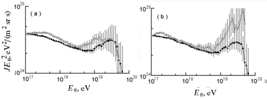
Figure 2. Integral energy spectra: a is for 28431 and 7504 showers with the arrival directions in the north ( \bullet ) and south ( \circ ) hemispheres of the Galaxy; b is for 3270 and 4234 showers with arrival directions -10^\circ < b_G < 0^\circ ( \bullet ) and b_G \leq -10^\circ ( \circ ).
