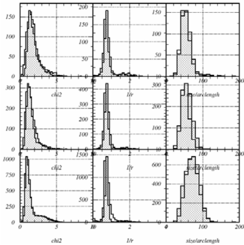
Figure 2. Observed muon parameters (histogram) compared with Monte Carlo simulations (hatched). From left to right, \chi^2 distributions for ring fitting, curvature distributions, and distributions of Size/Arclength , respectively. Upper, middle, and bottom panels are shown for T2, T3, and T4, respectively..
