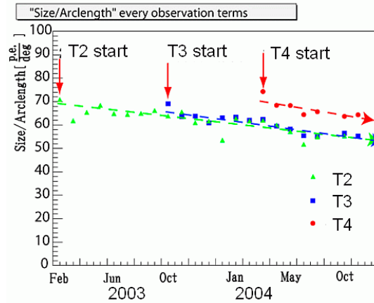
Figure 3. Time variation of the Size/Arclength for each telescope, which corresponds to the development of light collection efficiency.
