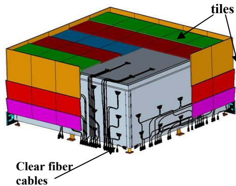
Figure 3. ACD detectors arrangement (4-th row tiles are not shown)
