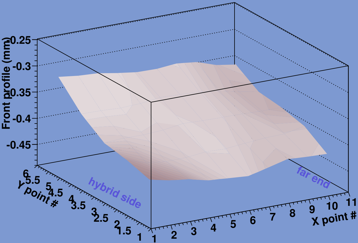
Rear Surface Profile Along Module 20220130000011
