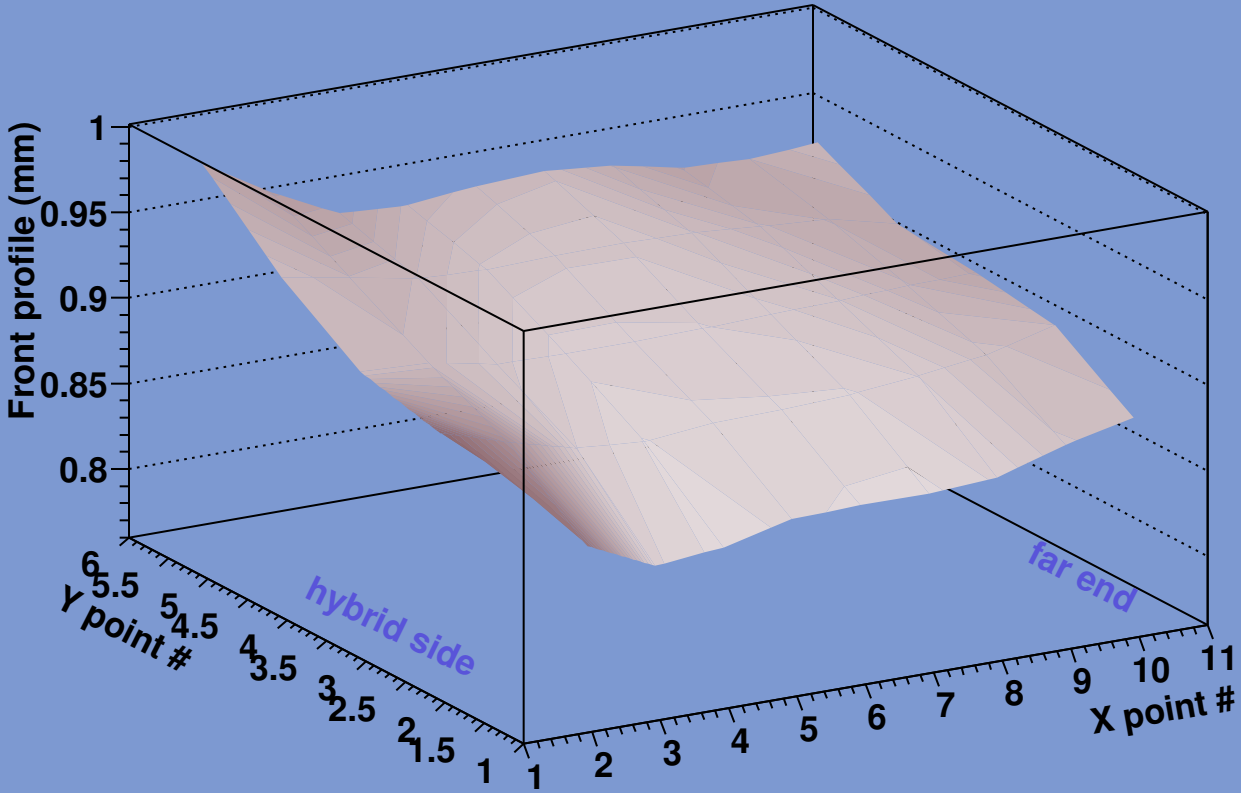
Front Surface Profile Along Module 20220130000011
