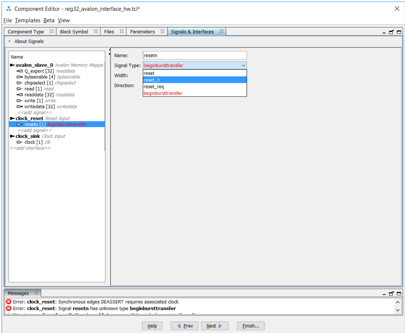
Figure 19. Specifying the signal type for resetrn .
