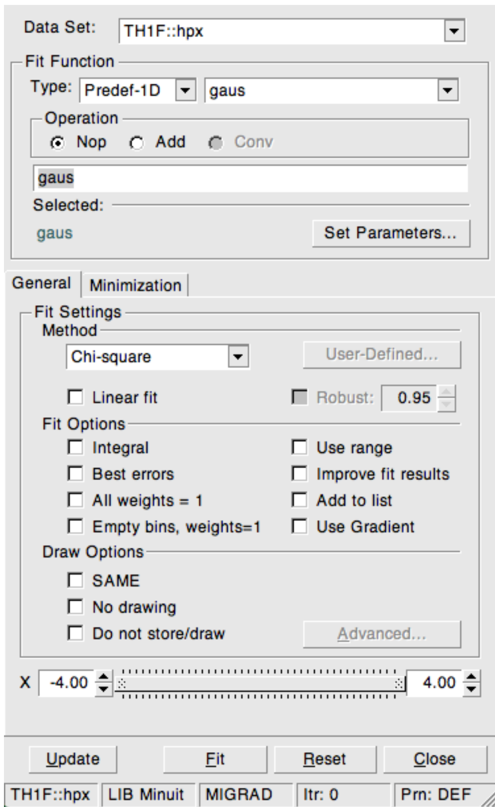
Figure 2.5: Fit Panel.
