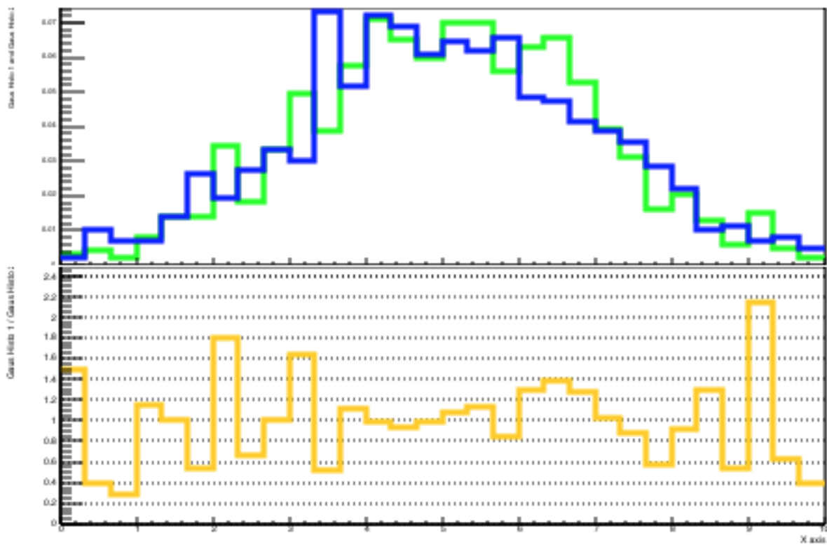
Figure 5.3: The ratio of two histograms.
